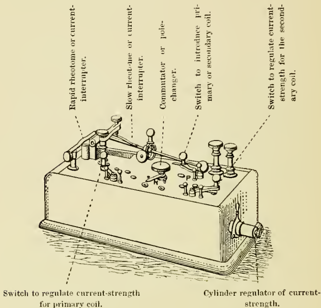
FARADIC APPARATUS FOR OFFICE TABLE.
